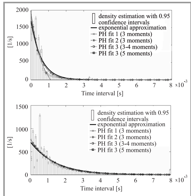
Fig. 5. Histograms of message inter-arrival times at the P-CSCF (top, c^2 = 2.19 ) and S-CSCF (bottom, c^2 = 1.33 ) CPU_i (data set 1, \lambda_{INV} = 100 [1/s]).
