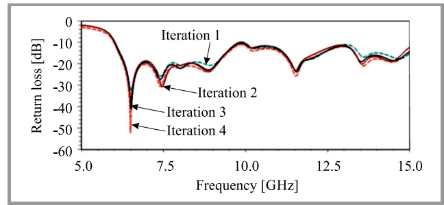
Fig. 4. Return loss comparison of each iteration. (For color pictures see the digital version of the paper).
