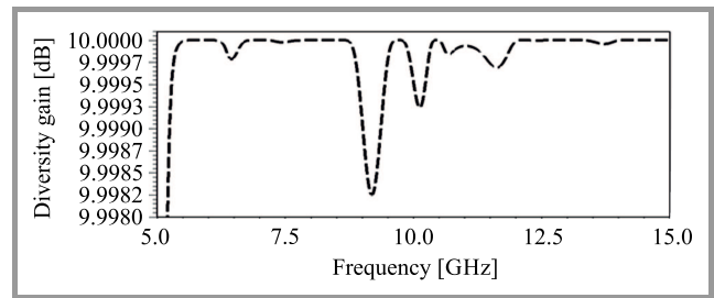
Fig. 13. Diversity gain.
